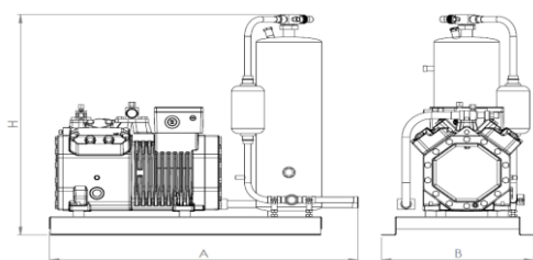
2EES-2Y/DVR500 - 4CES-9Y/DVR1500
