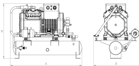
4TES-9Y/RHC15B - 6FE-50Y/RHC60B
